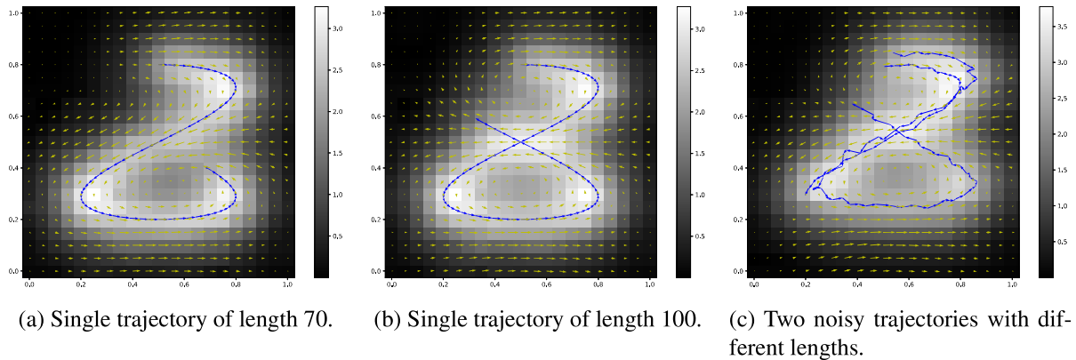
Figure 1: Observed trajectories (blue) and random field prediction at a regularly space grid (yellow). The gray background represents the uncertainty associated with the prediction.
