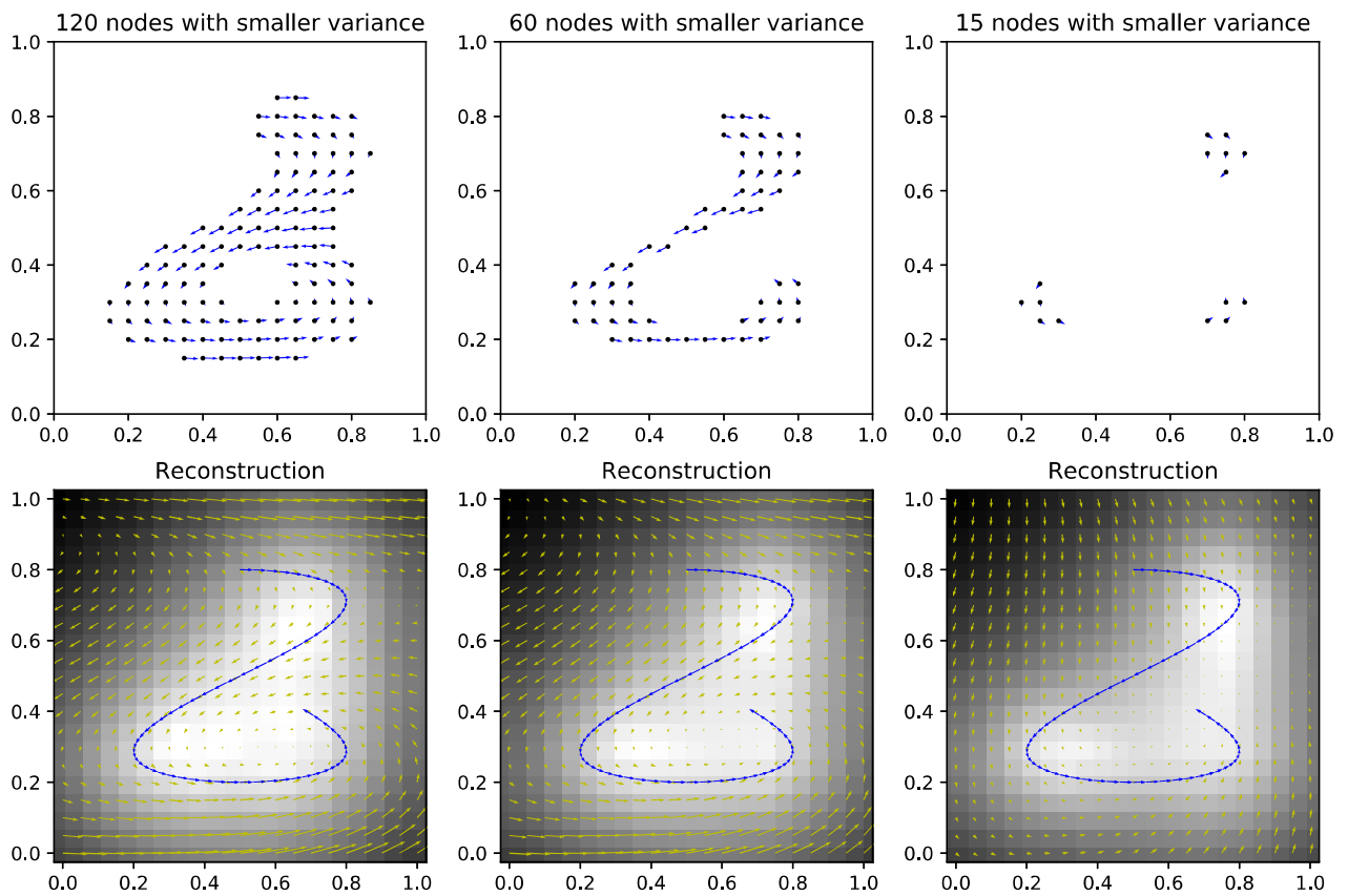
Figure 2: Observed trajectory (blue) and random field prediction at a regularly space grid (yellow). The gray background represents the uncertainty associated with the prediction.
