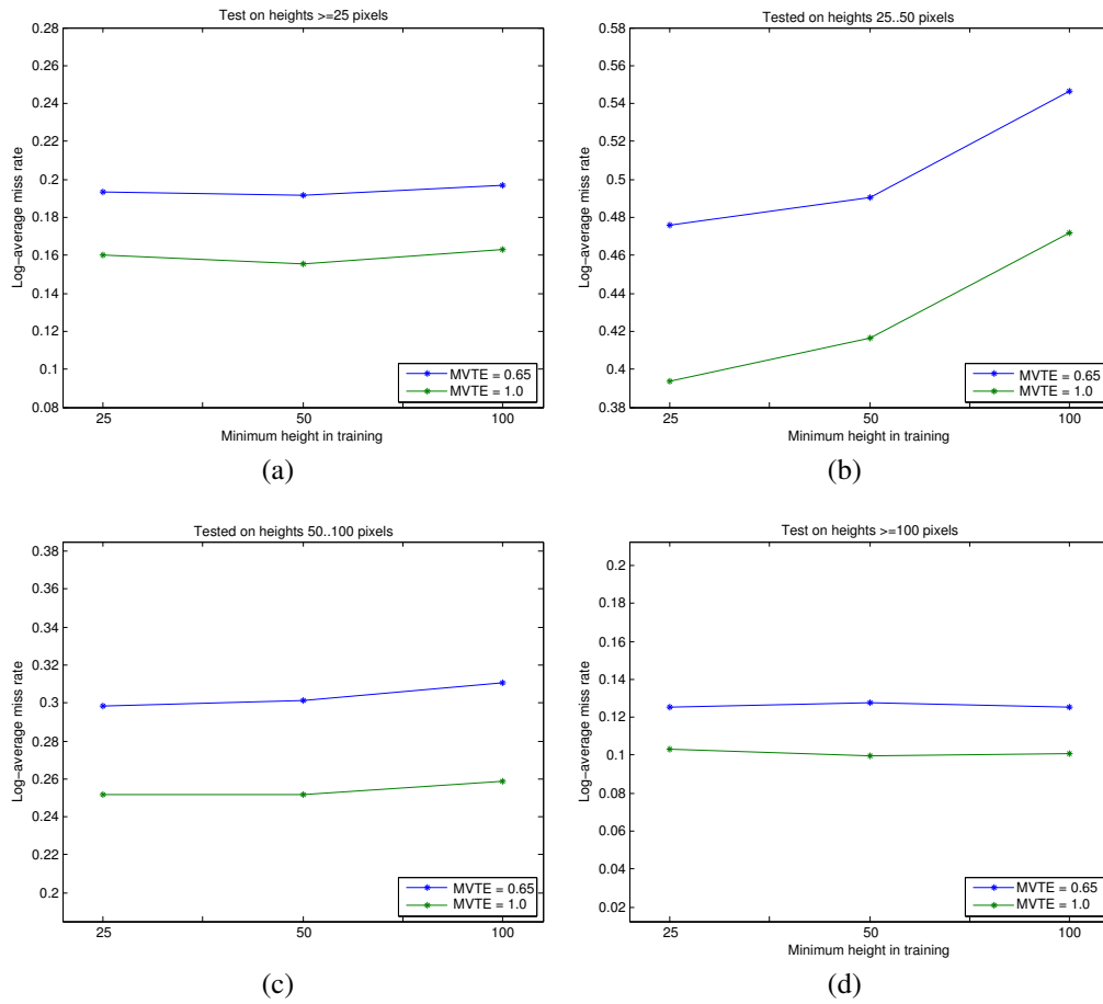
Figure 10. Log-average miss rate obtained varying minimum training height, ACF detector. The four plots display the results obtained with two test modes: full visibility (MVTE = 1.0) in green and minimum visibility in testing (MVTE) of 0.65 in blue. (a) When testing on pedestrians spanning the whole range of heights, the different training conditions fail to produce different performances. (b) When testing on short pedestrians, it is important to include examples of similar size in the training. Including examples of medium height is also advantageous. (c) When detecting medium height pedestrians it works to include “middle sized” pedestrians in the training set, but including the small ones does not help. Including the smaller pedestrians doesn’t change much the detection performance on the big pedestrians (b). Overall, since in the INRIA test the pedestrians with heights under 50 pixels are just 47 out of 879, the improvement of detection accuracy on this range has a small impact on the accuracy measured on the full test set (c).
