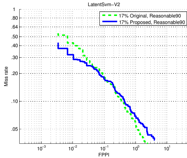
Figure 6. The reported performance of the LatSvm-V2 algorithm [27] using the original and the proposed labelling, in green and blue respectively. The evaluation mode is “Reasonable90” in both cases. Performance is summarized in the legend with the Log-Average Miss Rate. Using the proposed annotation instead of the original one reports considerably lower Miss Detection rates at low FPPI values. We ascribe this effect to the pedestrians that are unlabelled in the original annotation and have been labelled in the proposed one: the corresponding detections are evaluated as False Positives with the original annotation and as True Positives with the proposed one. Using the proposed annotation also reports slightly increased Miss Detection rates at high FPPI values. We attribute this effect to the introduction in the test set of more occluded pedestrians, which are arguably more difficult to detect than the fully visible ones.
