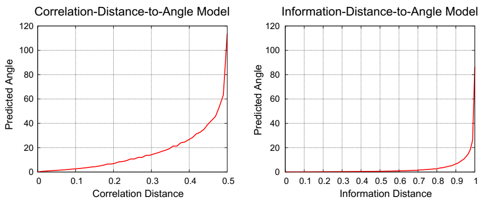
Fig. 7. Models relating correlation (left) or information distance (right) to angular separation between photocells. These models were built from simulated signals produced by the linear probe of Fig. 4(a). Signals of length T = 135,900 , acquired indoors were used.
