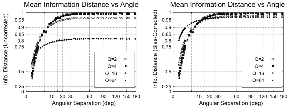
Fig. 6. Dependency of the information distance d(i, j) on the angular separation \theta_{ij} . The height of each plotted point is the average of 100 estimates of the information distance between signals x(i, 1 \leq t \leq 1359) and x(j, 1 \leq t \leq 1359) . The abscissa is the angular separations between pixels i and j of the discrete camera. Each curve corresponds to a different number Q of quantization bins. The quantization bins are all taken to have weight 1/Q . Right: Information distances computed with the first-order bias correction term of Eq. (4) removed. Left: Distances computed without correction.
