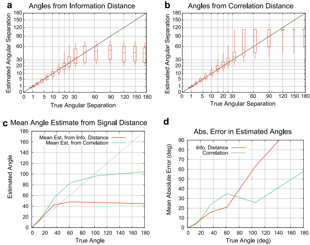
Fig. 8. Validation of the distance-to-angle models of Fig. 7. Boxplots (a) and (b) show the 5th percentile, first quartile, median, third quartile and 95th percentile of 100 angles estimated from signals of length T = 1359 simulated using the indoor sequence of Fig. 4(c). The angles are estimated from information distance in (a) and correlation in (b). The curves in (c) show the mean estimated angle vs. the true angle, and (d) shows the mean absolute error in the estimated angles.
