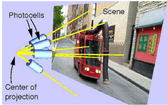
Fig. 1. A discrete camera consists of a number of photocells (pixels) that measure the light traveling along pencil of lines. More generally, one could consider that each photocell is characterized by a point spread function defined on the 3D sphere.
