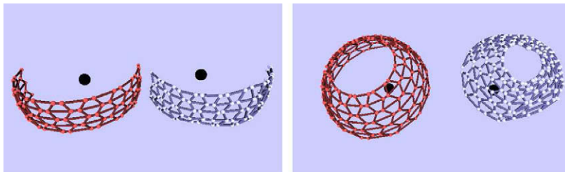
Fig. 13. Calibrations of two different sensors covering more than one hemisphere. On the left, a band-like sensor consisting of 85 photocells, calibrated from correlations (estimated: smaller, true: bigger). On the right, a discrete camera covering more than 180^\circ \times 360^\circ , of 168 photocells, calibrated from the information distance (estimated: smaller, true: bigger). Each ball represents a photocell except the big black balls, representing the optical center.
