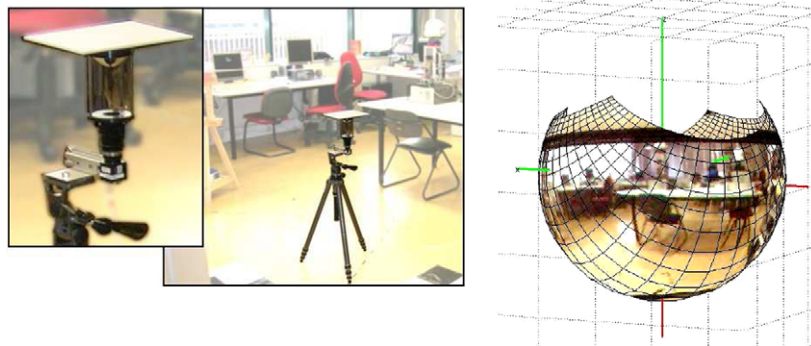
Fig. 3. Left: The camera used to sample omnidirectional images (image mirrored). Right: A calibrated omnidirectional image mapped to a sphere.
