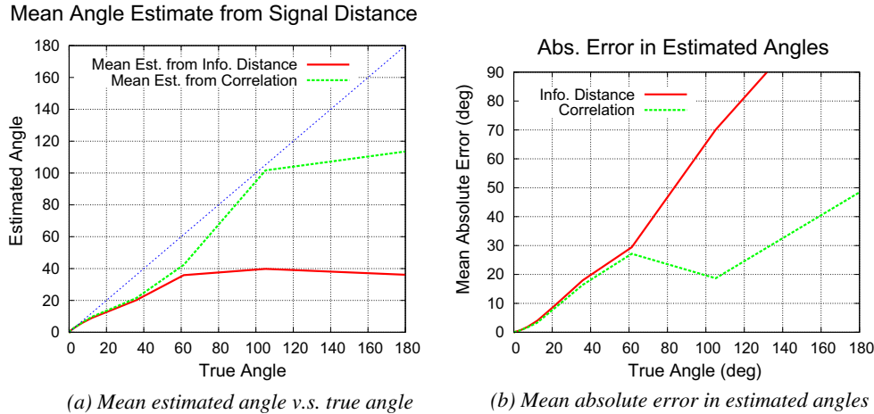
Fig. 10. Results of the angle estimators estimated from the sequence of Fig. 9, but with the virtual linear sensor kept mostly horizontal. (a) Mean of 100 sets of angles, plotted versus the true angle. (b) Mean absolute error in the estimated angles.
