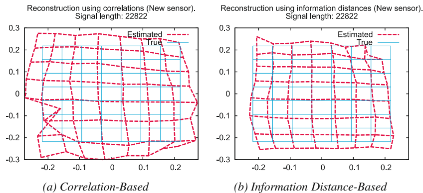
Fig. 14. Reconstructed and true pixel layouts of a discrete camera consisting of photocells lying on a rectangular grid (a and b). The sensor used differs from that with which the models of Fig. 6 were built. The reconstructions are obtained by first estimating the pairwise angular distances, then embedding the angles in the sphere (see text). For visualization, the reconstructions are aligned by the usual procrustes method, mapped to the plane by projective mapping with unit focal length. Added line segments show the true pixel neighborhood relations. Plot (a) is obtained from the correlation distance, and plot (b) from the information distance.
