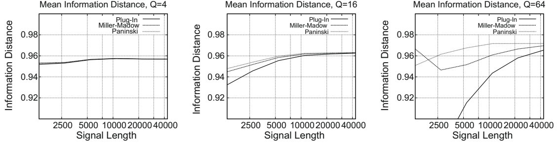
Fig. 5. Each of these plots shows how bias of various estimators is affected by signal length. Each curve is the average of 150 information distance estimates, taken between signals generated by photocells separated by approximately 5^\circ . The signal length is varied from 1359 to 43488. A good estimator is one for which the mean value changes little with the signal length. The three considered information distance estimators are: the plug-in estimator, the Miller–Madow corrected estimator and Paninski’s estimator.
