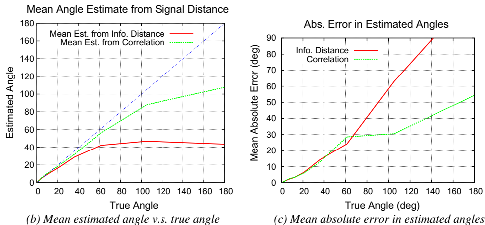
Fig. 9. (a) Four out of 2349 images of an outdoors and indoors sequence used to validate the angle estimators. (b) Mean of 100 sets of angles estimated from this sequence, plotted versus the true angle. (c) Mean absolute error in the estimated angles.
