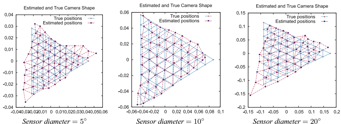
Fig. 12. True and estimated pixel layouts of a discrete camera consisting of photocells lying on a triangular grid. To estimate the layout, each pixel was sampled 1359 times. The information distance between pairs of pixels was estimated from these values, and converted to angular estimates using our non-parametric model. The angular distances were then embedded in the sphere. For visualization, they are aligned by the usual procrustes method, mapped to the plane by projective mapping with unit focal length, and line segments indicate the original pixel neighborhood relations.
