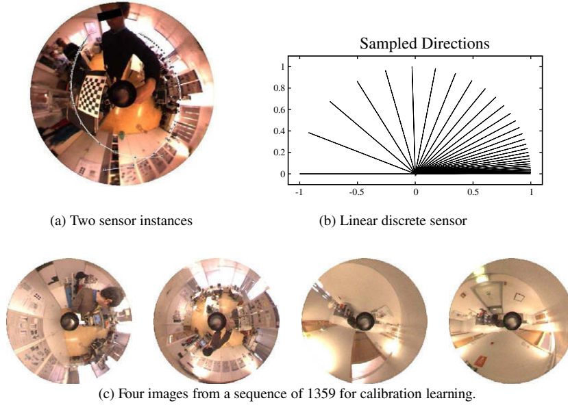
Fig. 4. (a) Two instances of the linear discrete camera, inserted in an omnidirectional image. Pixels locations are indicated by small crosses connected by white lines. (b) Geometry of a discrete camera consisting of a planar array of thirty one (31) pixels, spanning 180^\circ in the plane. The first two pixels are separated by 0.5^\circ , the separation between consecutive photocells increases geometrically (ratio \approx 1.14 ), so that the 31st photocell is antipodal with respect to the first. (c) Four images of a set to be used for calibration learning.
